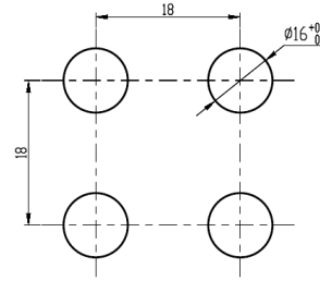
Mounting hole sizes
