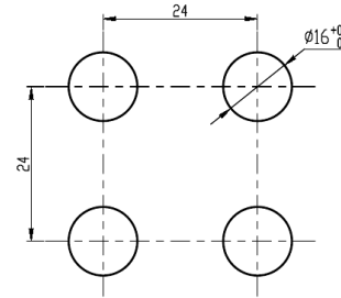
Mounting hole sizes
