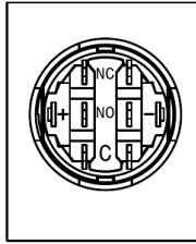
Terminal description
